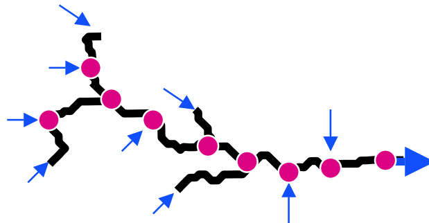
Figure A1.3: A typical river network in the Topnet model. Runoff from catchments (blue arrows) enters the river network either at the head of small streams, or at node points within the river network.
