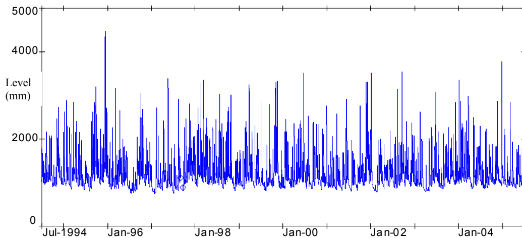
Figure 5: Lake level data for Lake Moeraki, measured every 15 minutes (levels are relative to a local datum). The rapid changes in level caused by rain events are large, in comparison to the differences between levels on 1 July each year.
