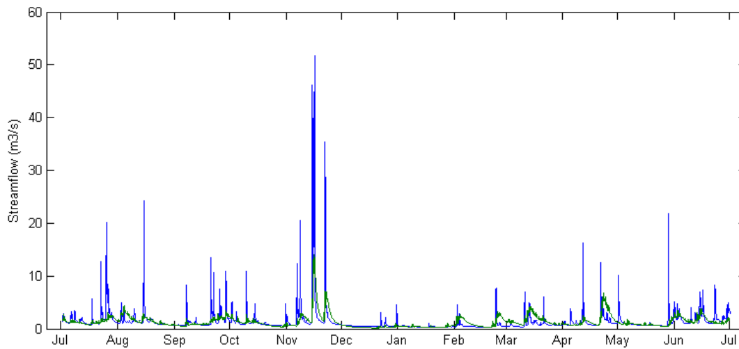
Figure 3: Topnet model validation for 1994-95 on Punehu Stream at Pihama in Taranaki (thick line is measurement, thin line is model). Using an uncalibrated Topnet model, the modelled mean flow is 9% smaller than the measured mean flow.
