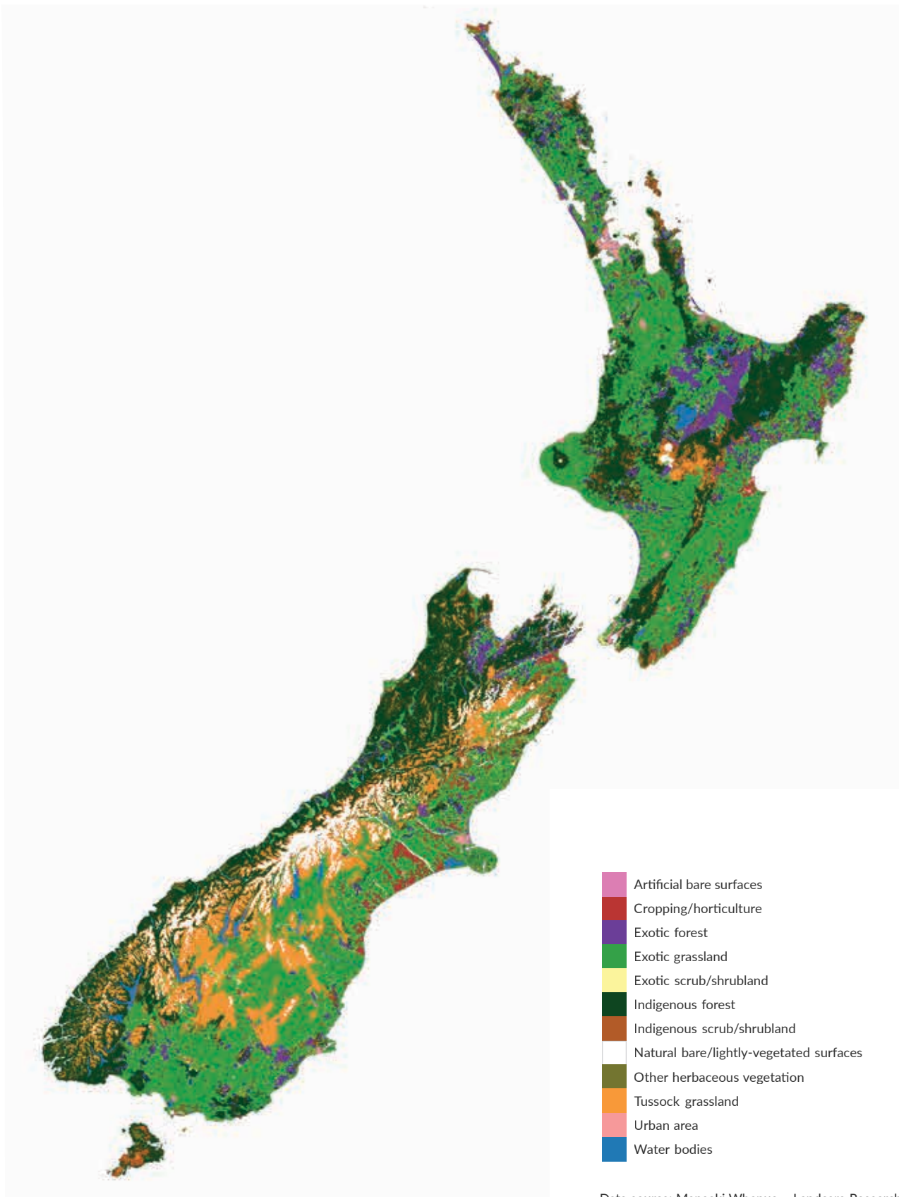
Figure 4: Land cover, 2012
